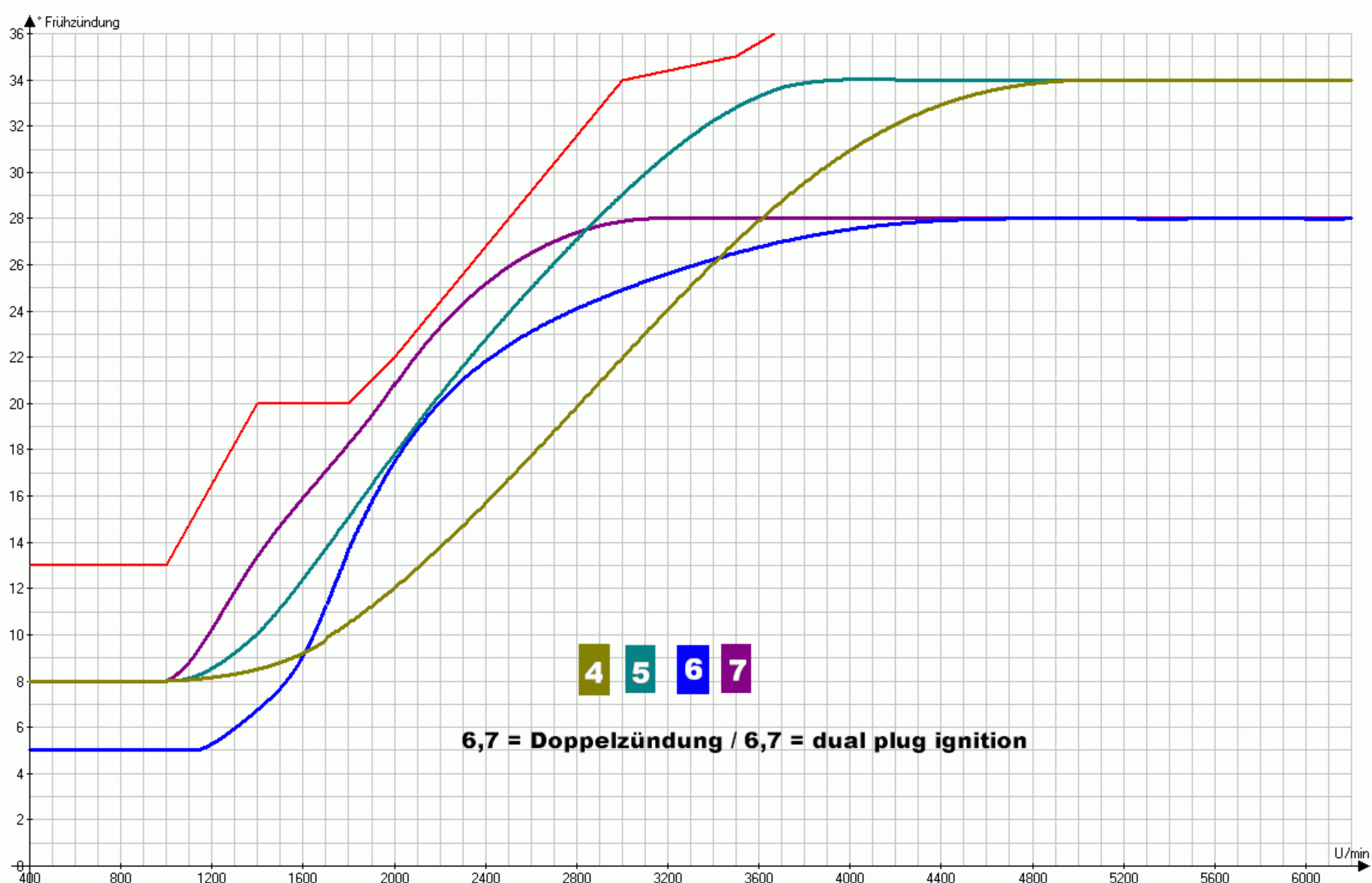
Kurven/diagrams 4-7
